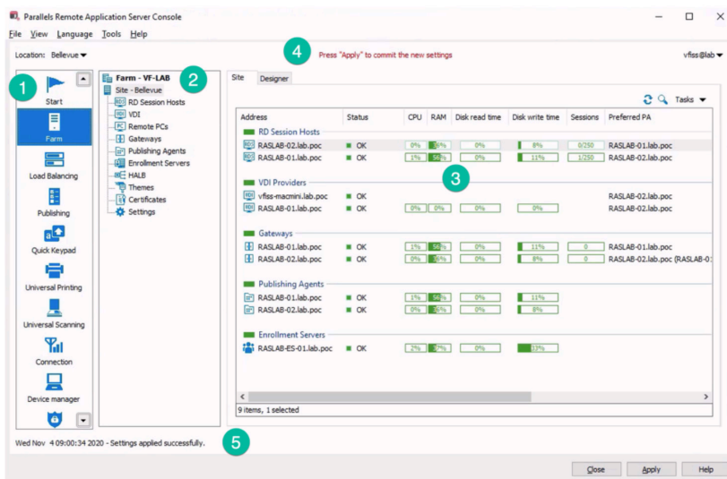
Figure 3. Parallels Remote Application Server Console general overview
